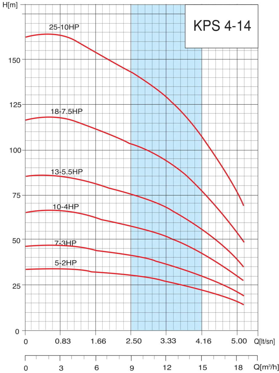
KPS 4-14 SERİSİ PERFORMANS TABLOSU KPS 4-14 SERIE PERFORMANCE TABLES
